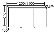
SPLA120/140 SPLB120/140*
