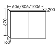
SPIY060/080/100 SPIZ060/080/100*
