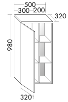
UHGZ050 UHAU050*
