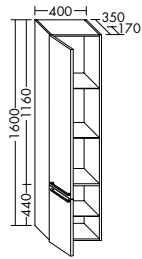
HSBJ040/HSBK040
